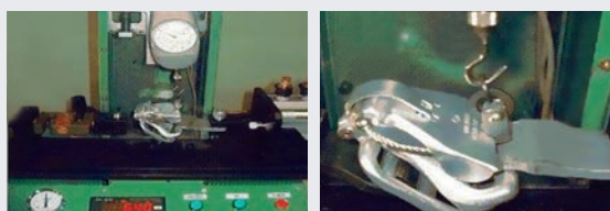
• COVER GUARD RELEASE TEST RELEASE AT 6~12 LBS
